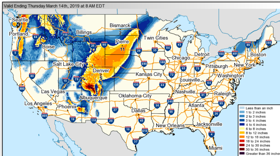
Forecast Snowfall
