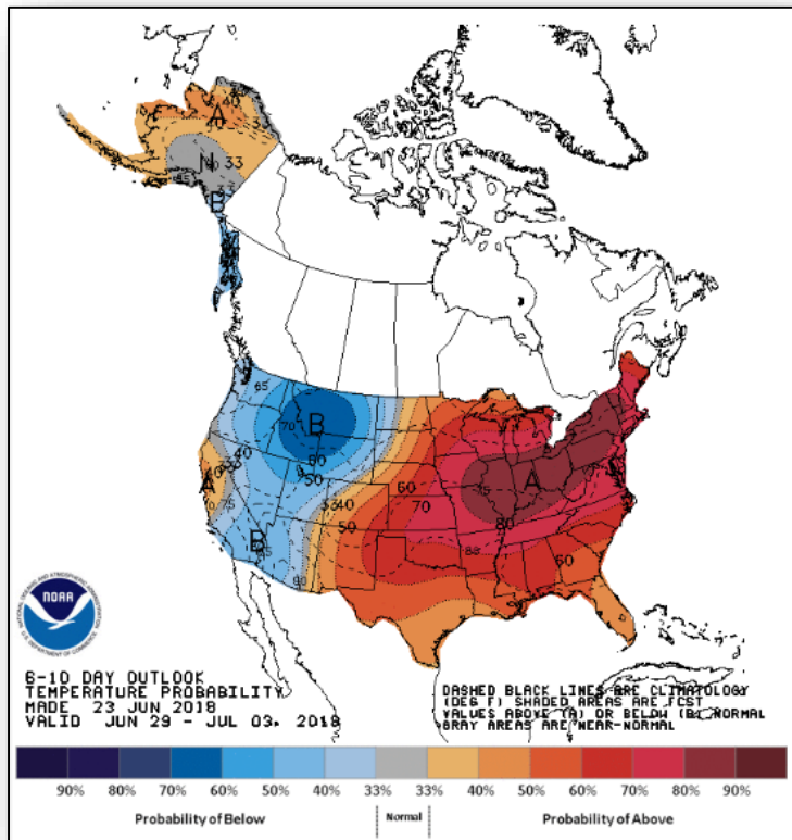
Temperature Probability
