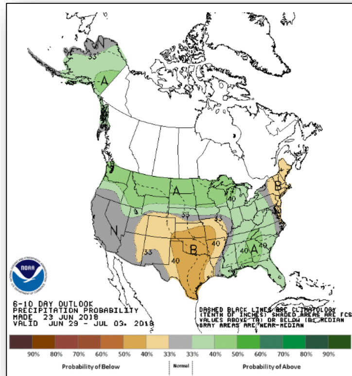
Precipitation Probability
